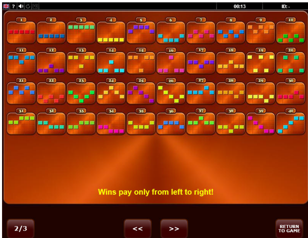
Help Screen 2
